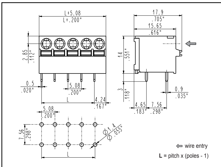
5.08mm Pitch Horizontal
