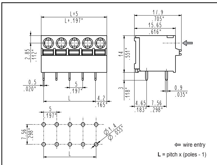
5.00mm Pitch Horizontal
