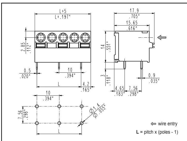
10.00mm Pitch Horizontal
