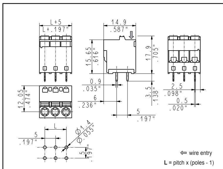
5mm Pitch Vertical
